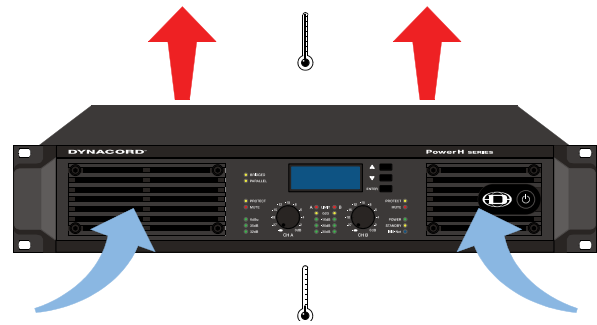
Illustration 2.6: H2500/H5000 Ventilation
